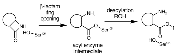
Scheme 3. The CAL-B catalyzed transesterification of \beta -lactams with alcohols proceeds in two steps: ring opening of the \beta -lactam followed by deacylation of the acyl enzyme intermediate.
