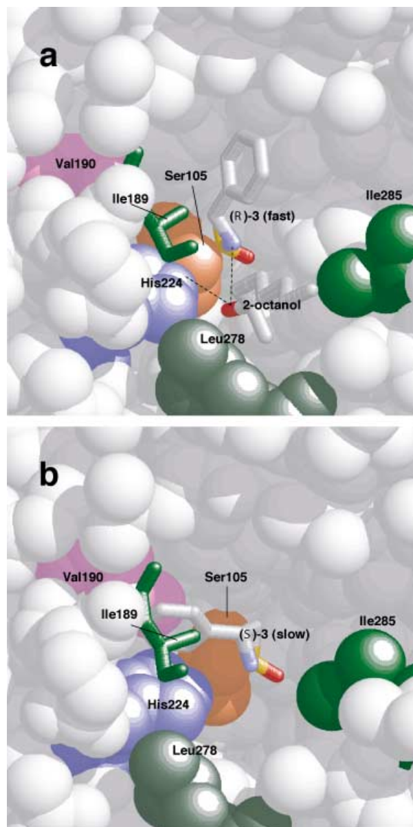
Figure 1. Proposed tetrahedral intermediate analogues of the enantiomers of \beta -lactam 3 . CAL-B is shown in space-filling representation, except for Ile189, which is shown as stick representations. The tetrahedral intermediate analogue for the \beta -lactam is shown in stick representation as is the 2-octanol in part a . a ) The proposed productive conformation for the fast-reacting enantiomer, ( R )- 3 , corresponds to structure c in Scheme 4. The phenyl ring points upward and toward the reader and makes good hydrophobic interactions with Ile189, Ala141, Thr138. b ) We did not identify any catalytically productive structures for the slow-reacting enantiomer, ( S )- 3 . The picture shows a non-energy minimized structure of the slow enantiomer in an orientation similar to that in part a . Upon energy minimization, the phenyl ring distorts to an unrealistic non-planar geometry due to severe steric clash with the side chains of Val190 and Ile189.
