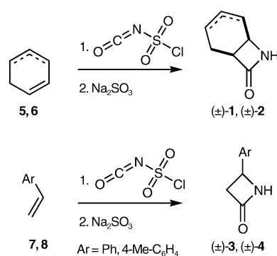
Scheme 2. Synthesis of racemic \beta -lactams.
