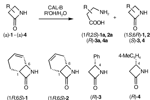
Scheme 1. Enantioselective ring opening of \beta -lactams yields a \beta -amino acid and unreacted \beta -lactam. The initial product may be the \beta -amino acid ester, but this ester hydrolyzes to the acid under the reaction conditions. The structures show the fast reacting enantiomers.
