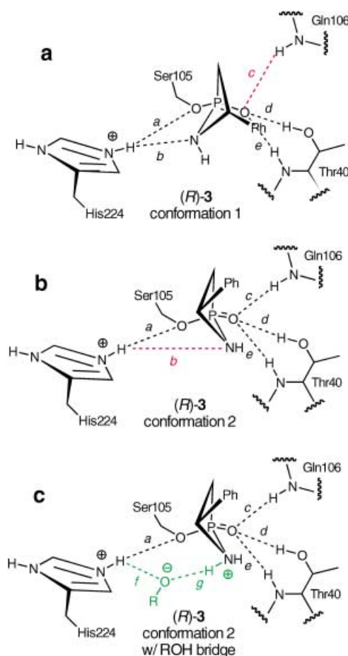
Scheme 4. Line diagrams of possible catalytically productive conformations for the ring opening of \beta -lactam ( R )-(+)- 3 (fast enantiomer) catalyzed by CAL-B showing the phosphonate analogues of the tetrahedral intermediates. a ) Conformation 1 orients the lactam amide towards His224. Hydrogen bond 'c' (red) between the main chain amide N–H of Gln106 and the phosphonyl oxygen, which mimics the oxyanion of the tetrahedral intermediate is weak or missing in this structure. In addition, the phenyl group encounters severe steric strain with Ile285 (not shown). b ) Conformation 2 orients the amide away from His224. Hydrogen bond 'b' (red) between His 224 N \epsilon –H and the \beta -lactam nitrogen is weak or missing. c ) The substrate alcohol forms a hydrogen-bonded bridge (green) between His 224 N \epsilon –H and the lactam nitrogen of conformation 2. This structure shows the alkoxide-bridged tautomer, but the alcohol-bridged structure is the same except the hydrogen being transferred (green) is on the oxygen of the alcohol. We propose that either the alkoxide-bridged or the alcohol-bridged structures are the catalytically productive conformations. (A sixth key hydrogen bond present in all structures is between His 224 N \delta –H and the carboxylate of Asp264. For clarity, neither this hydrogen bond nor Asp264 are shown in the line diagrams.)
